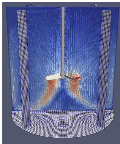
Figure 1 – Example of what your anaerobic digester model will look like.
